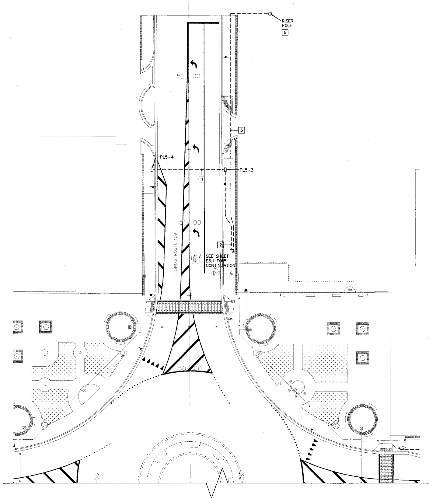
NORTH ELECTRICAL PLAN - POWER 1" = 20'-0"
