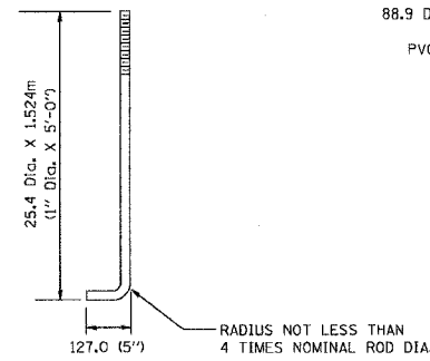
ANCHOR ROD DETAIL
