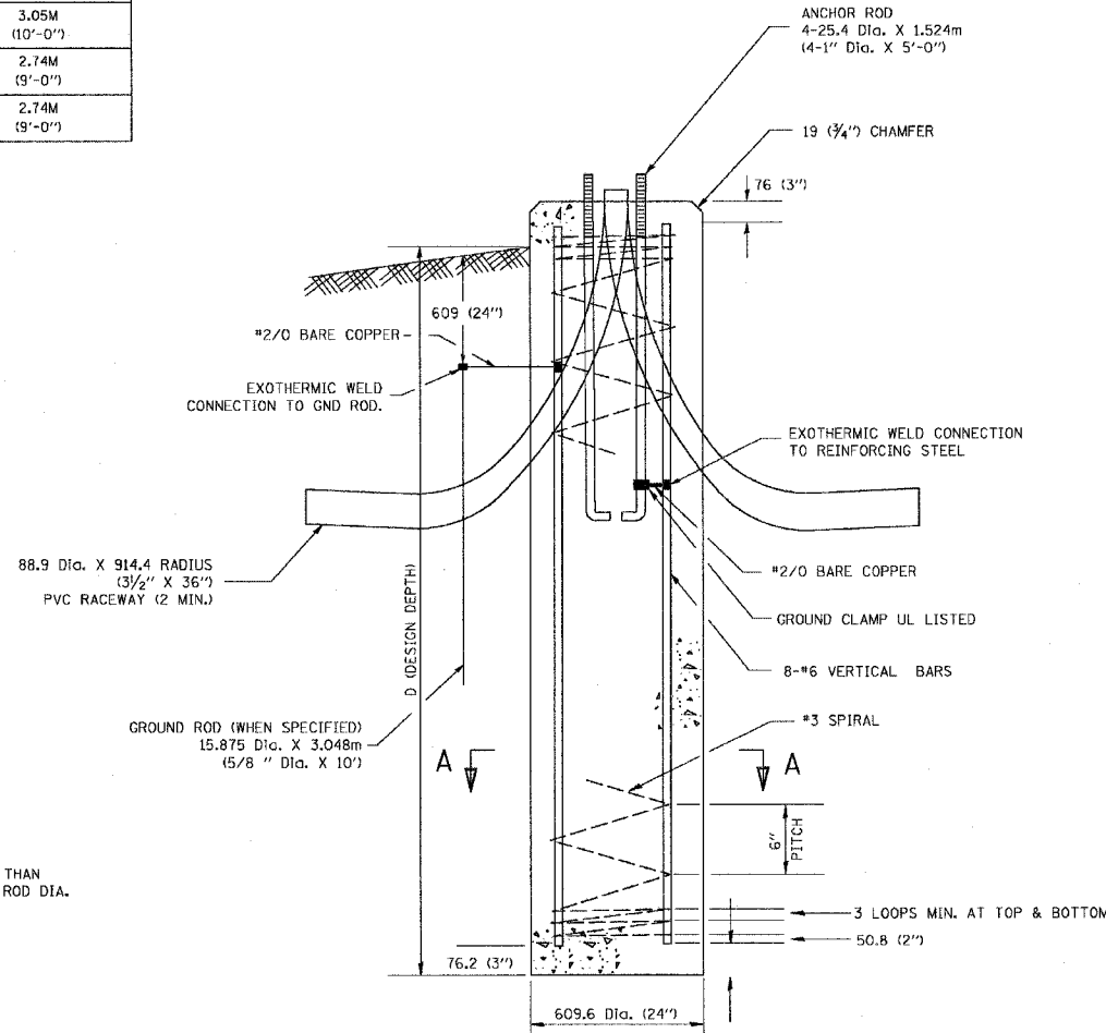
FOUNDATION DETAIL
