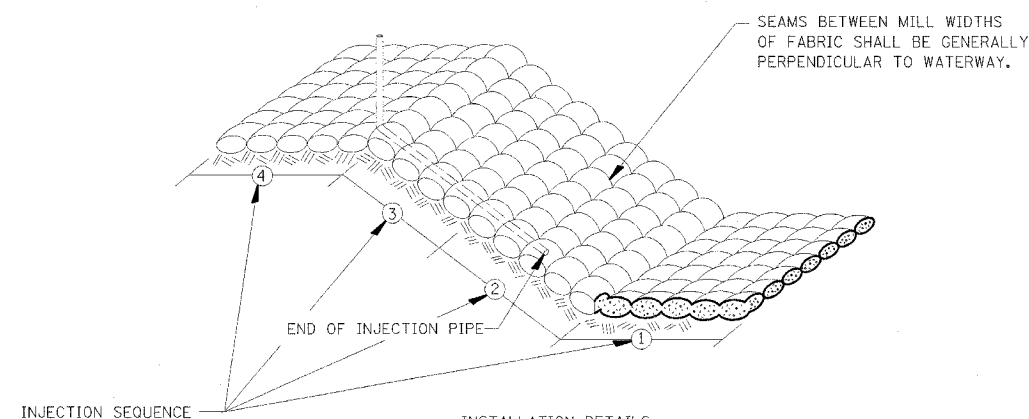
INSTALLATION DETAILS NOT TO SCALE
