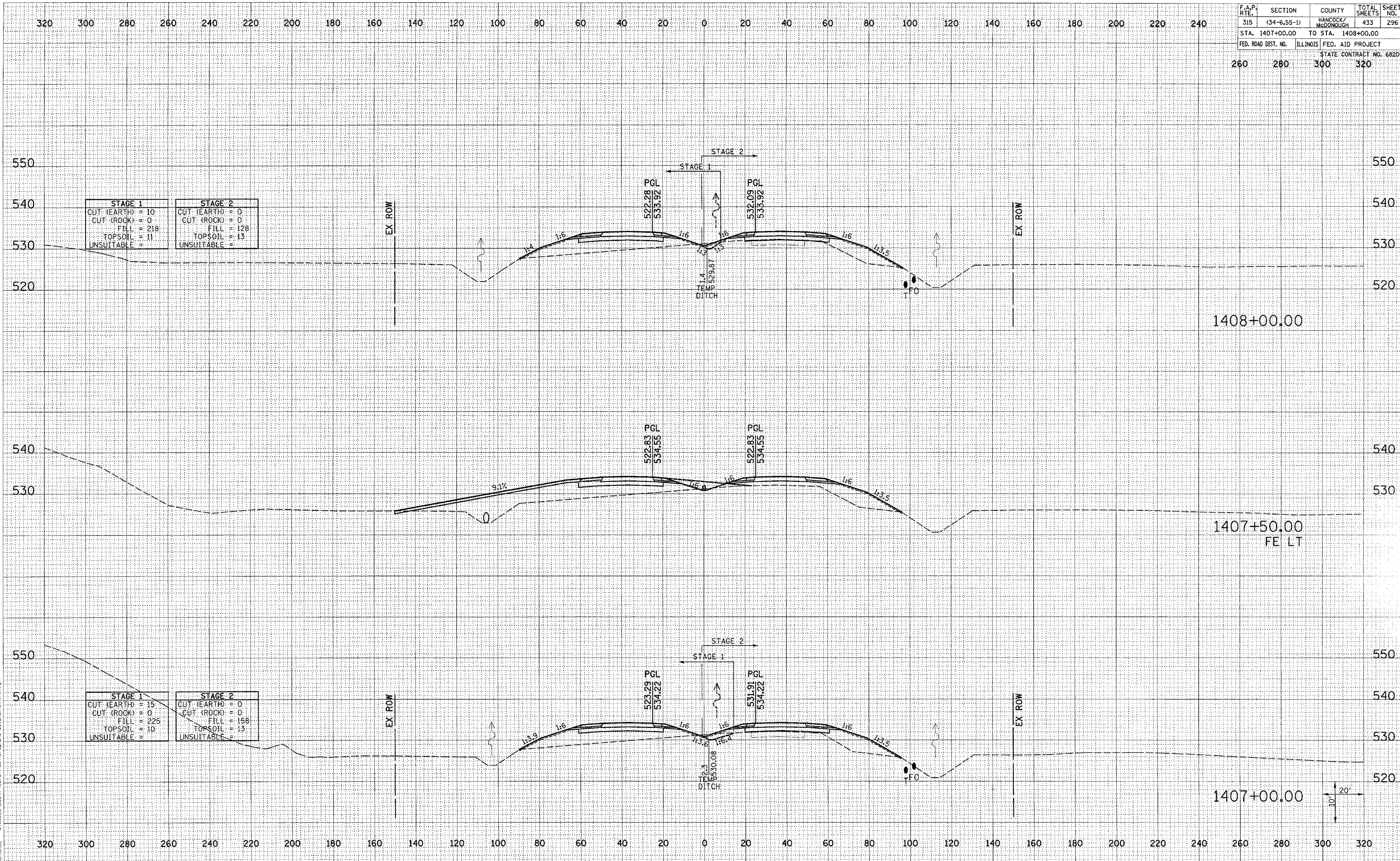
FAP ROUTE 315 (IL 336) CROSS SECTIONS STA 1407+00.00 TO 1408+00.00
