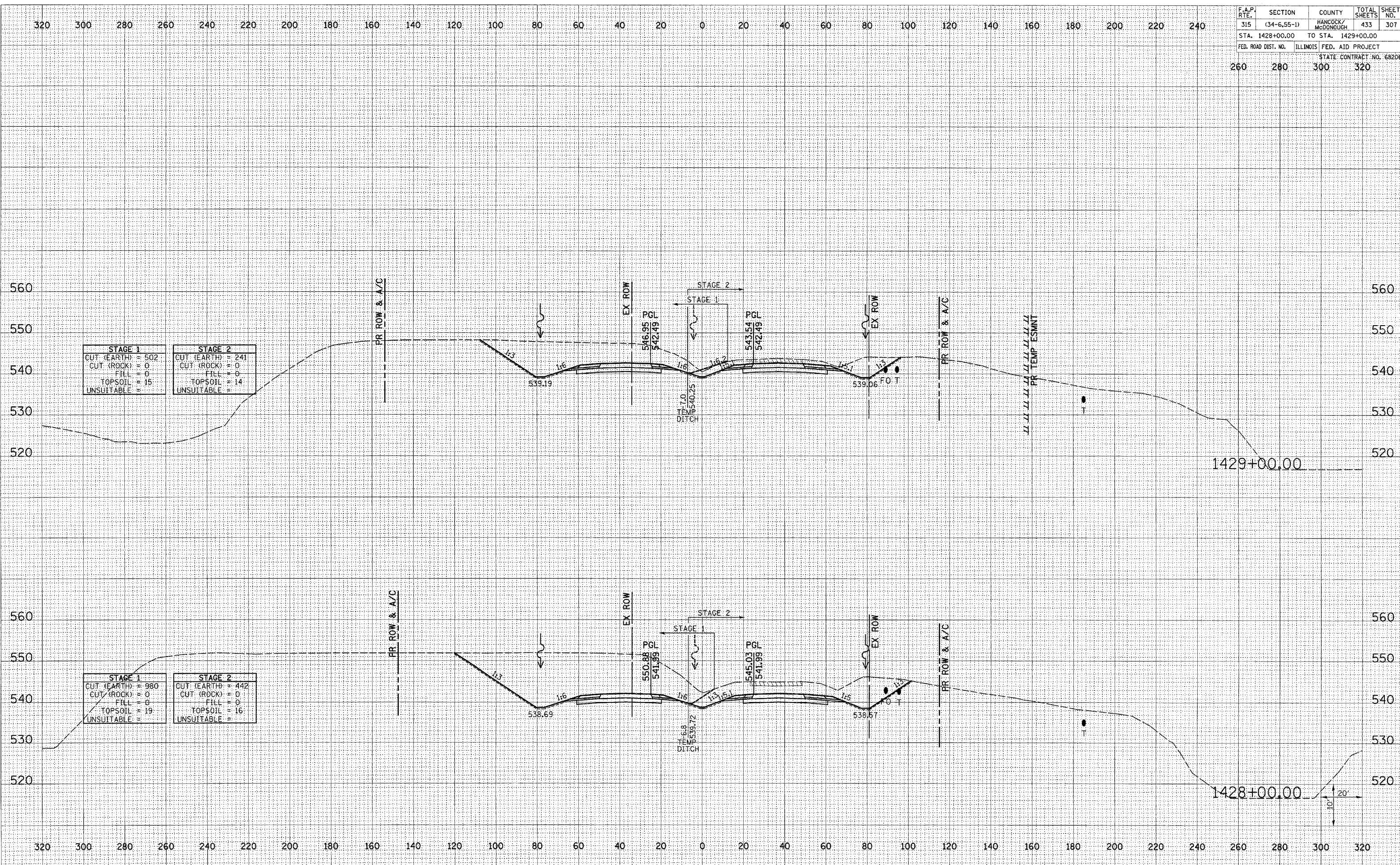
FAP ROUTE 315 (IL 336) CROSS SECTIONS STA 1428+00.00 TO 1429+00.00
