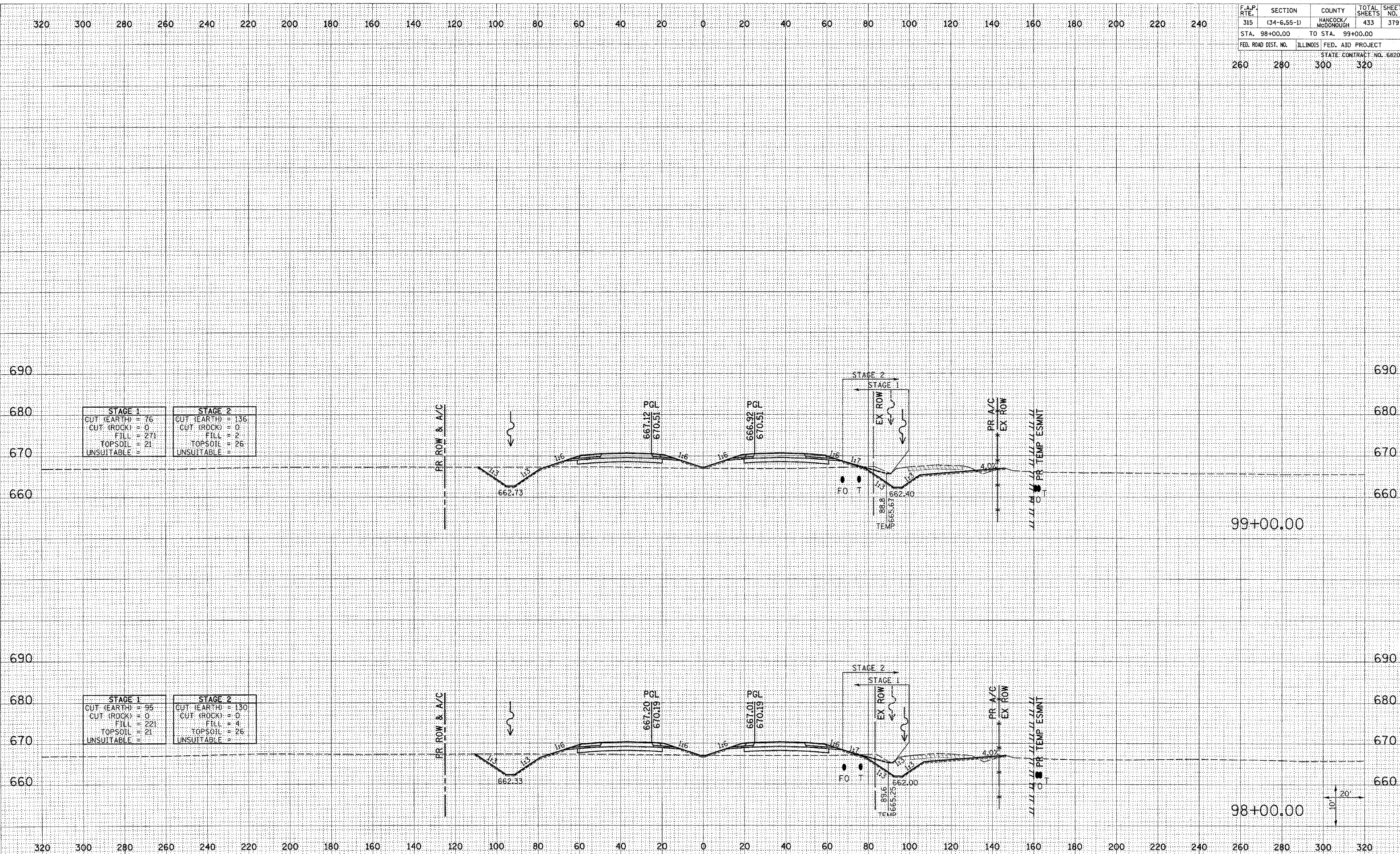
FAP ROUTE 315 (IL 336) CROSS SECTIONS STA 98+00.00 TO 99+00.00
