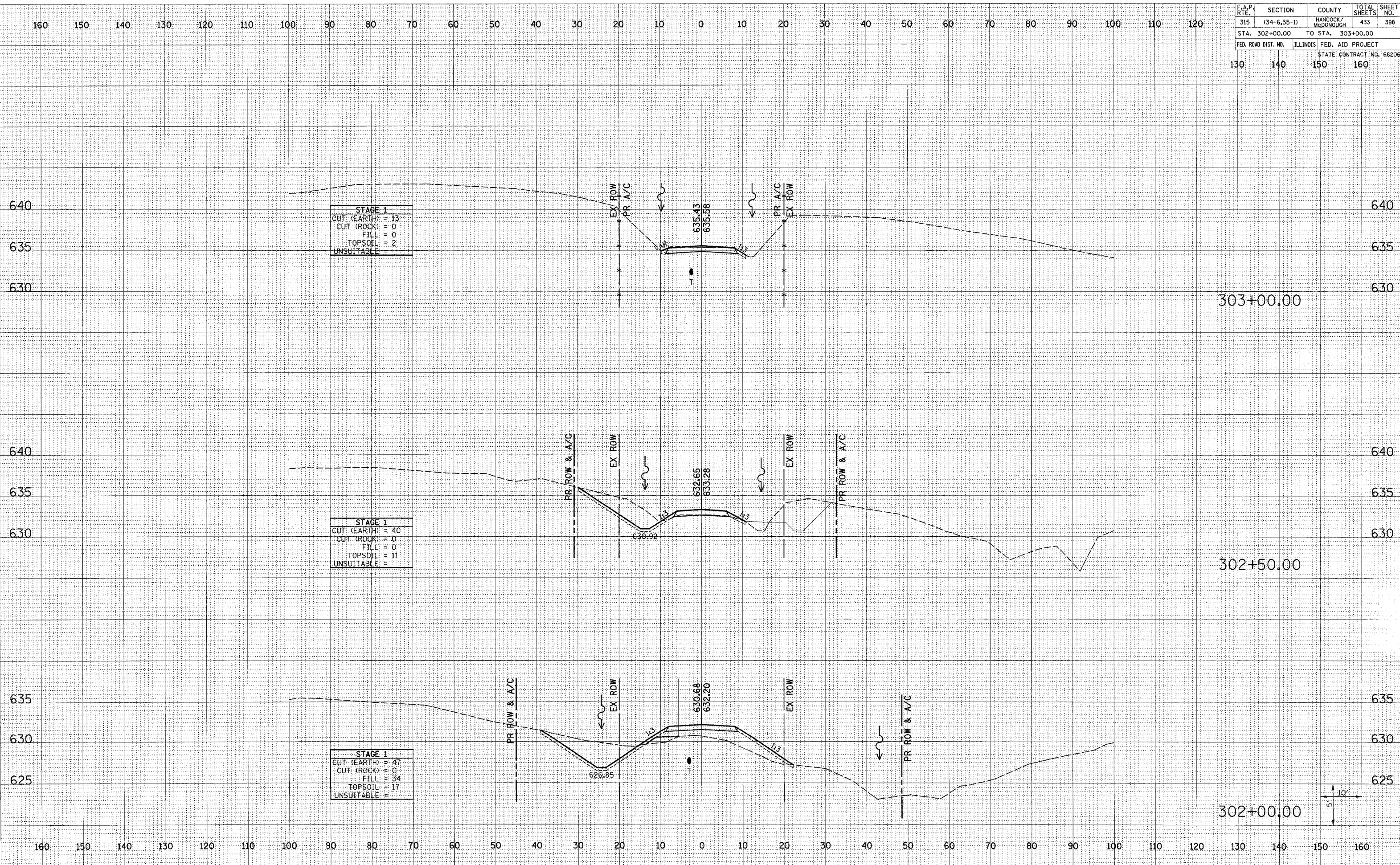
TR 257 CROSS SECTIONS STA 302+00.00 TO 303+00.00
