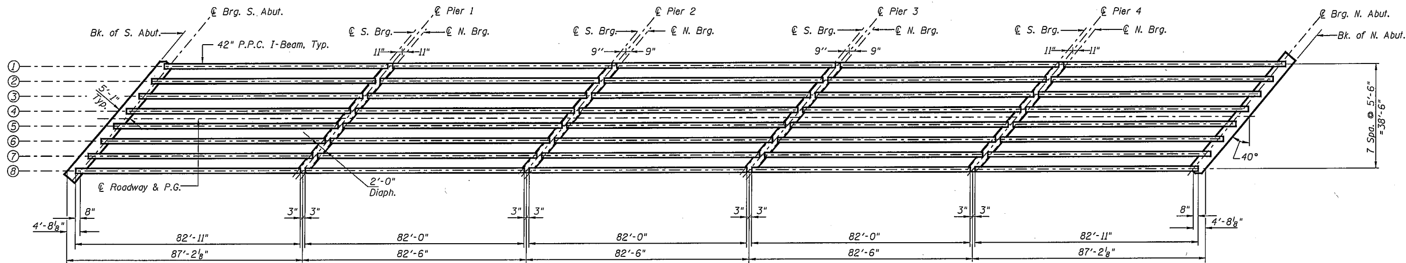
FRAMING PLAN
