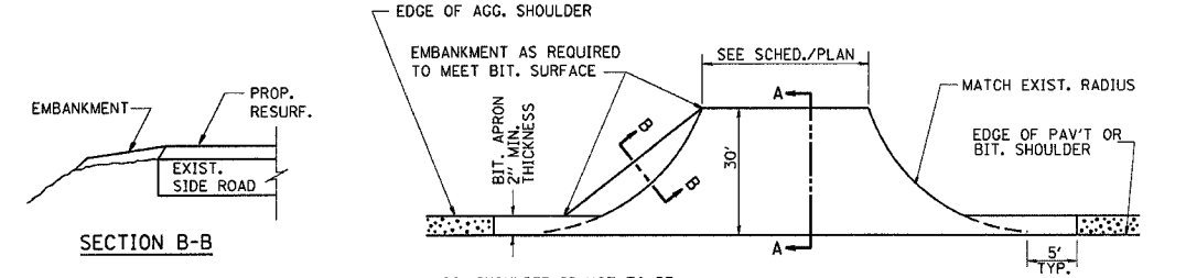
PLAN AT SIDE ROADS
