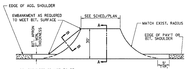
PLAN AT SIDE ROADS
