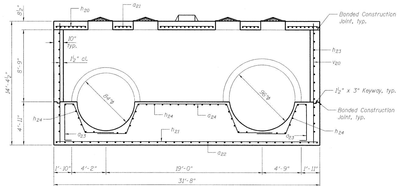
SECTION E-E
