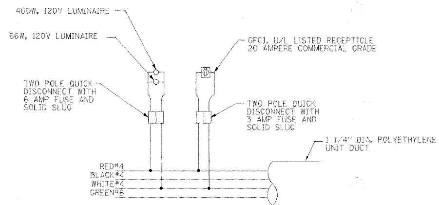
SINGLE POLE WIRING
