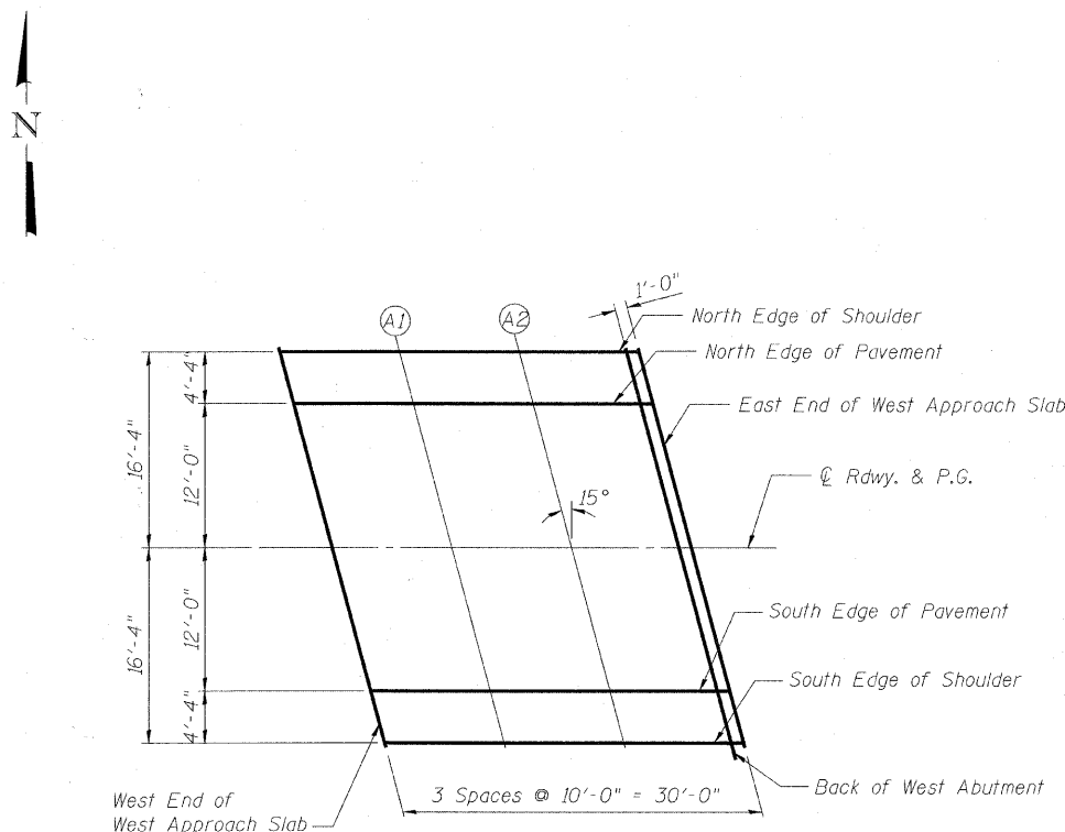
PLAN West Approach
