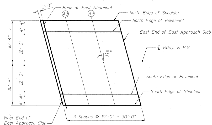
PLAN East Approach
