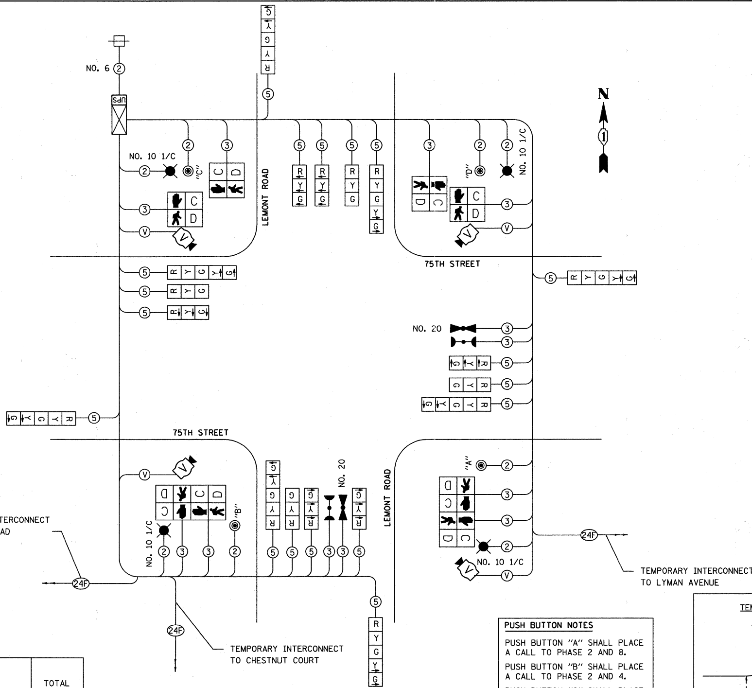
TEMPORARY CABLE PLAN FOR STAGE 3 NOT TO SCALE
