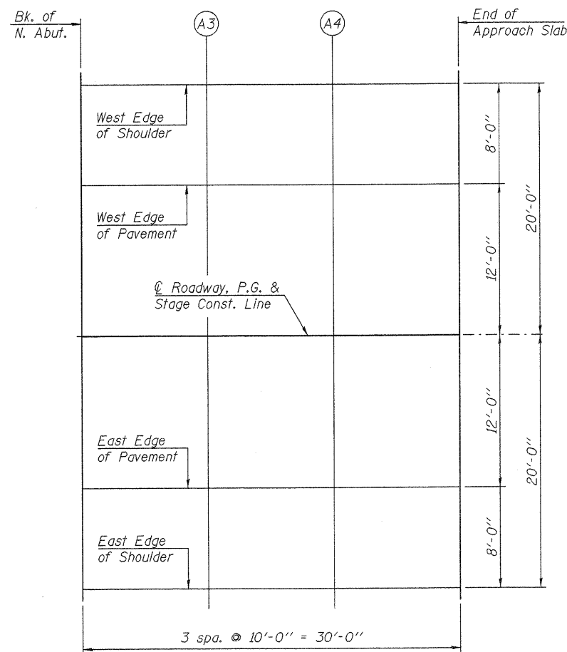
PLAN
