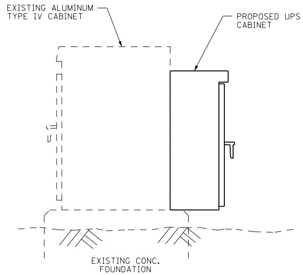
TYPICAL UPS MOUNTING (SIDE VIEW)
