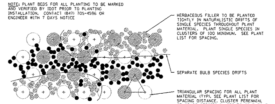
INTERPLANTING DETAIL - MULTIPLE BULB SPECIES
