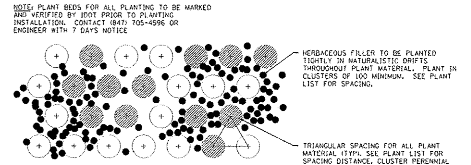
INTERPLANTING DETAIL - SINGLE BULB SPECIES
