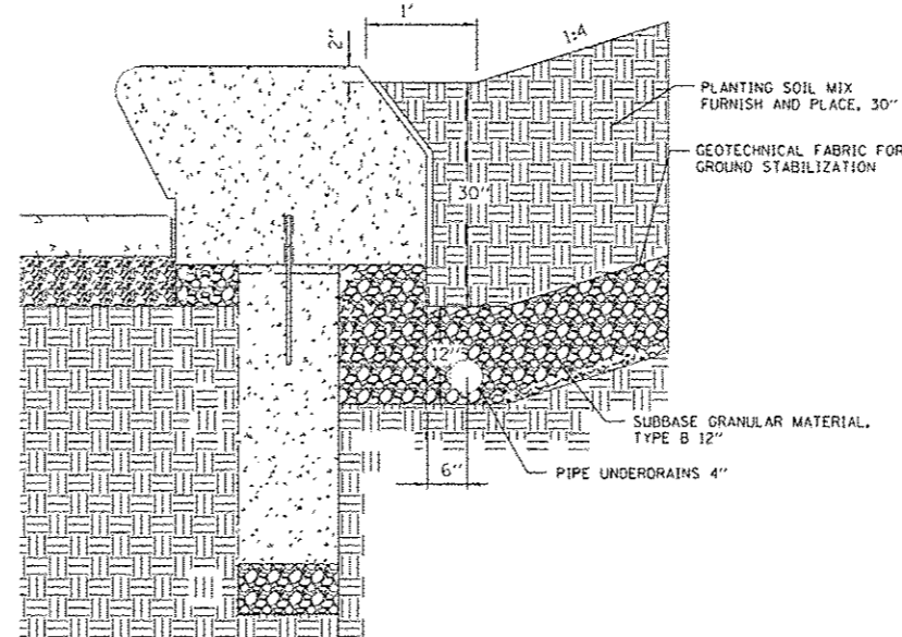
WALL DETAIL NOT TO SCALE
