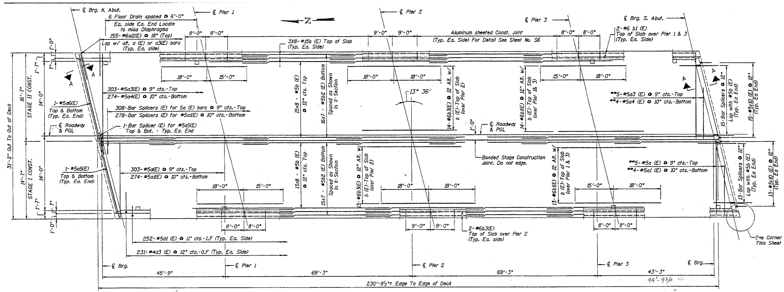
DECK PLAN
