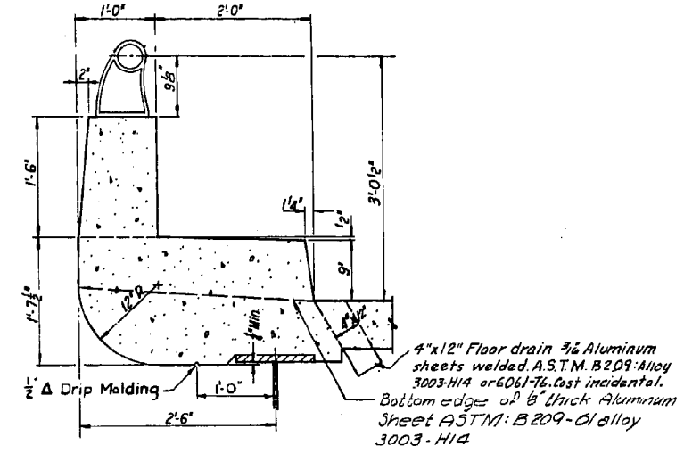
CURB DETAIL
