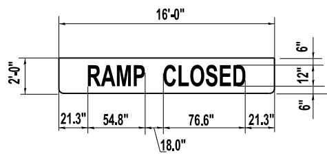
TEMPORARY SIGN TO COVER EXISTING SIGN 16'X2'
