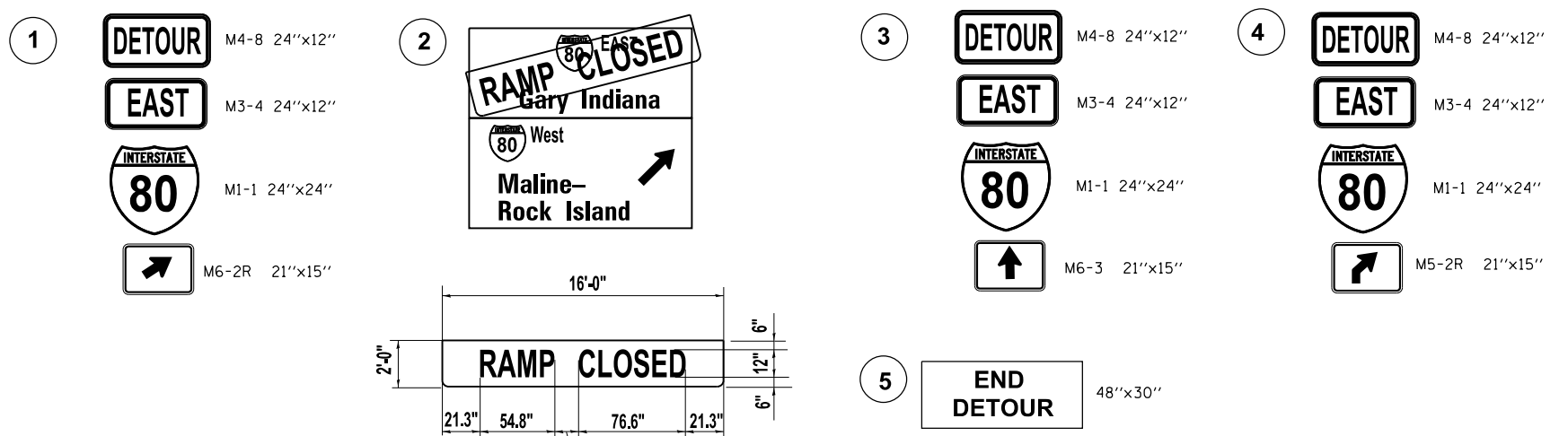
TEMPORARY SIGN TO COVER EXISTING SIGN 16'X2'
