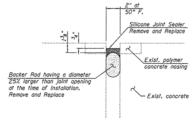
SECTION THRU EXPANSION JOINT (Typ. for SN 084-0143, 0144, 0145, and 0146)
