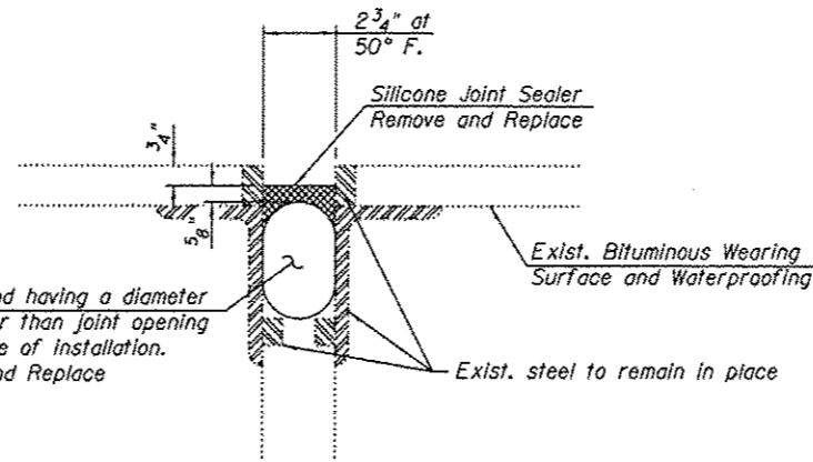
SECTION THRU EXPANSION JOINT (Typ. for SN 084-0140, SN 084-0141 similar.)
