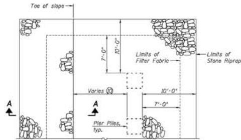
RIPRAP PROTECTION AT PIER
