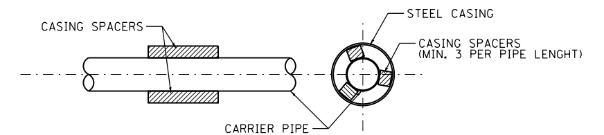
CASING SPACER DETAIL NOT TO SCALE
