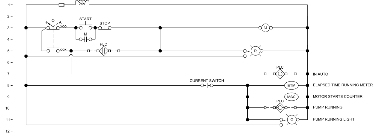
CONTROL DRAWING No. 9
