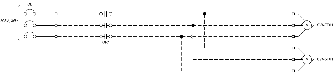
CONTROL DRAWING No. 8
