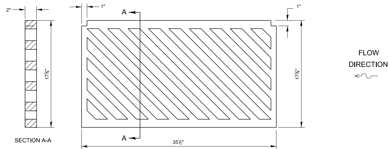
PLAN VIEW OF CAST IRON GRATE 1 3/8" DIAGONAL BARS WITH 1 1/4" OPENINGS
