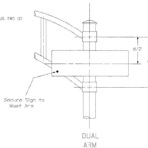
SIGNFIX ALUMINUM CHANNEL FRAMING SYSTEM Shd be used. See Note #5.
