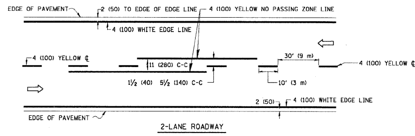
2-LANE ROADWAY
