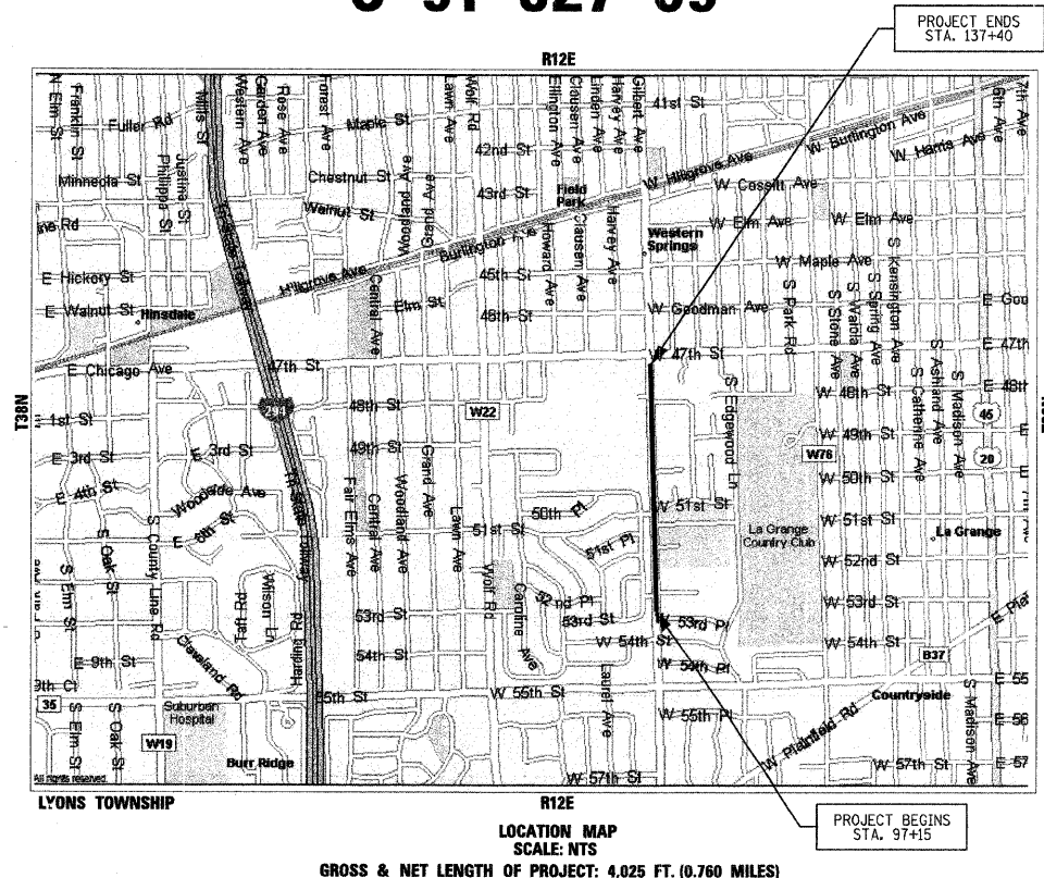
GROSS & NET LENGTH OF PROJECT: 4,025 FT. (0.760 MILES)
