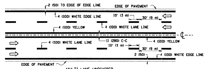
MULTI-LANE UNDIVIDED
