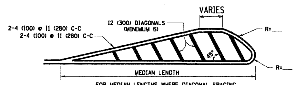
4' (1.2 m) WIDE MEDIANS ONLY
