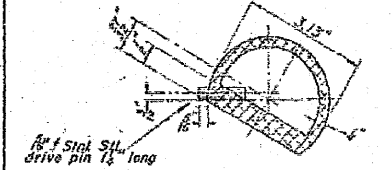
SECTION THRU SPLICE TOP RAIL
