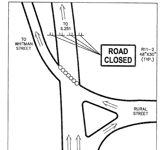
CLOSURE DETAIL
