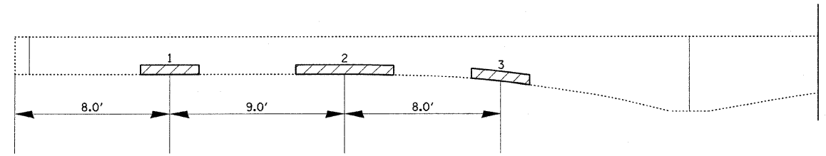
051-0017 NORTH OUTSIDE FACIA BEAM EAST ABUTMENT (LOOKING SOUTH)
