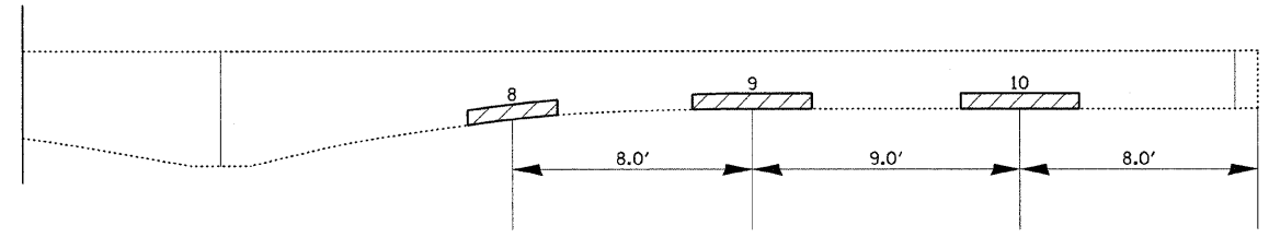
051-0017 NORTH INSIDE FACIA BEAM EAST ABUTMENT (LOOKING NORTH)
