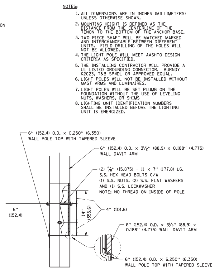
DAVIT ARM CONNECTION [14\"/>
