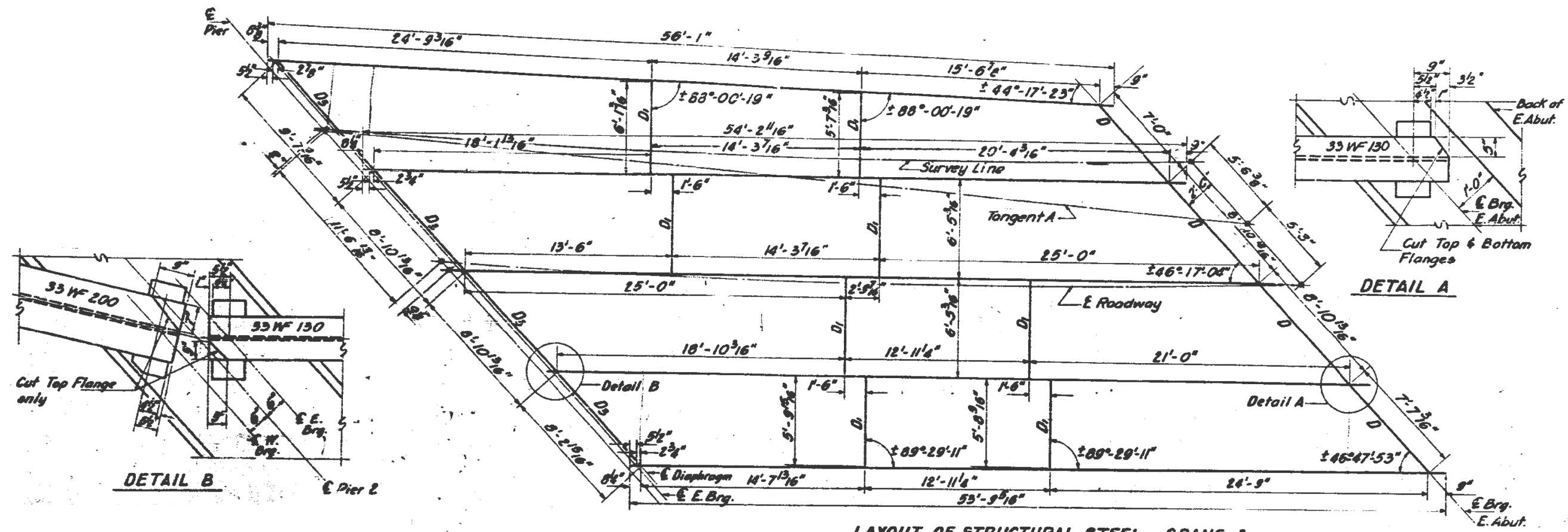
LAYOUT OF STRUCTURAL STEEL - SPANS 3 (All Beams 33 WF 130)
