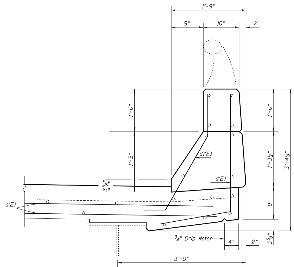
SECTION A-A (Dimensions at RT L's to end of deck)
