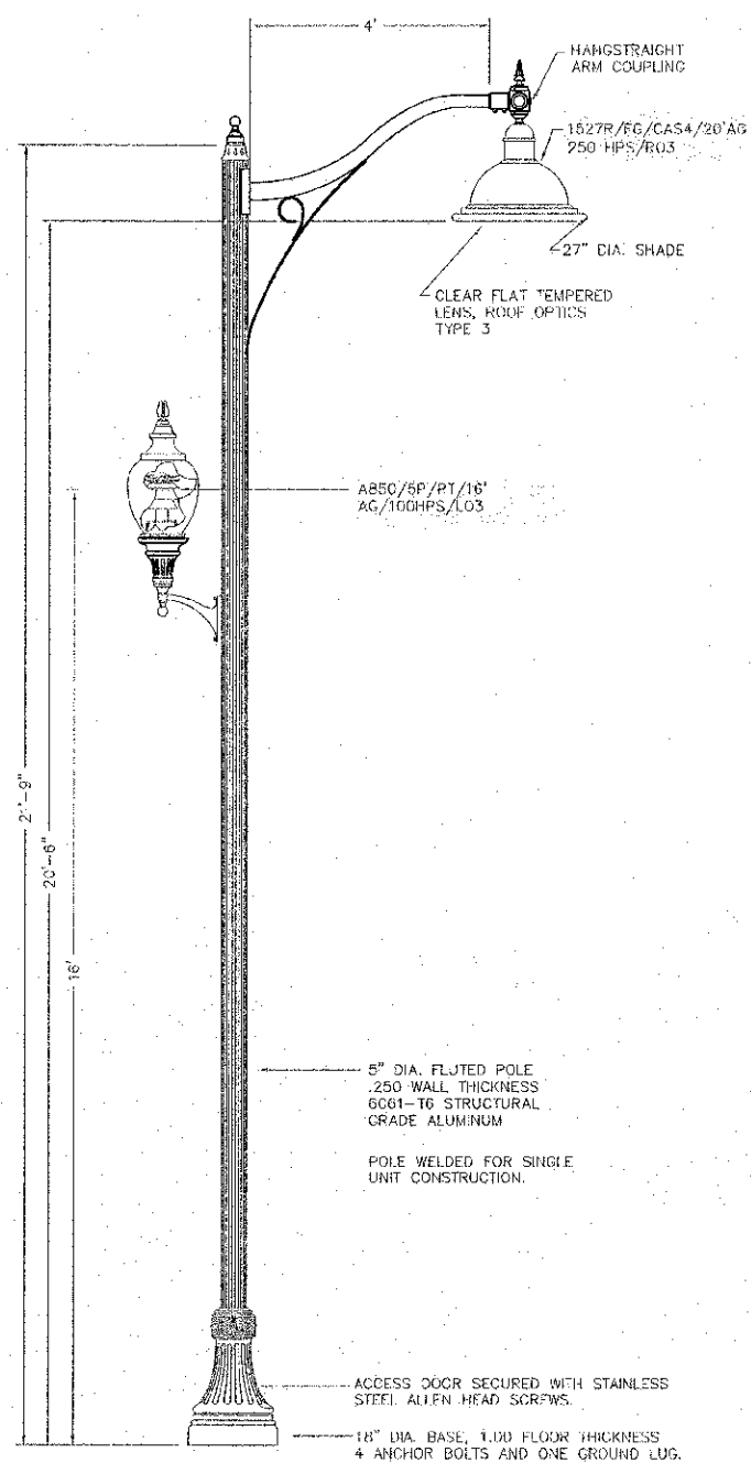
STREET & SIDEWALK LIGHT "OR APPROVED EQUAL"
