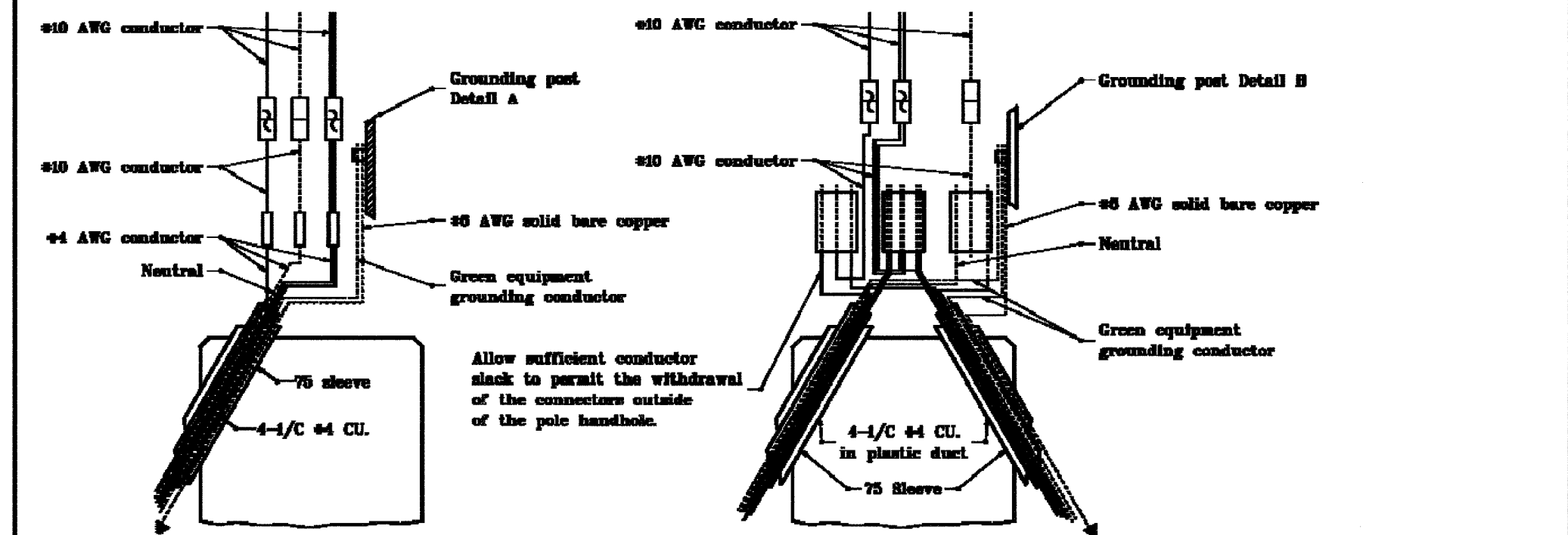
OVERHEAD SIGN SERVICE DETAIL (UNDERGROUND CONNECTIONS)
