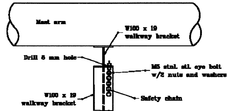
DETAIL B
