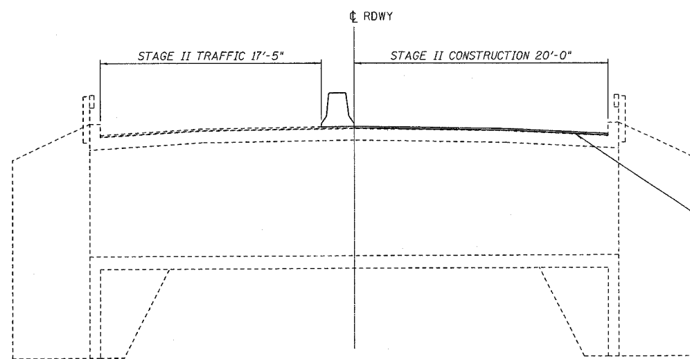
STAGE II CONSTRUCTION
