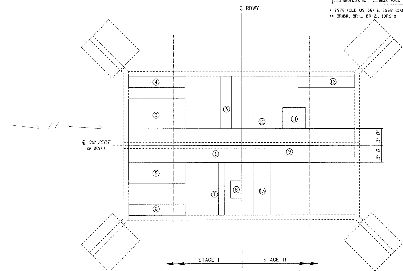
DECK SLAB REPAIR PLAN
