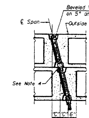
PARTIAL PLAN TRANSVERSE TIE ASSEMBLY (D=0°, 5° and 10°)
