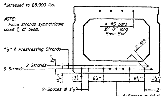
CROSS SECTION (50' SPAN)
