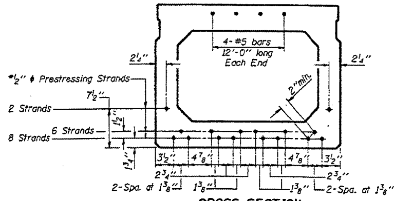
CROSS SECTION (60' SPAN)
