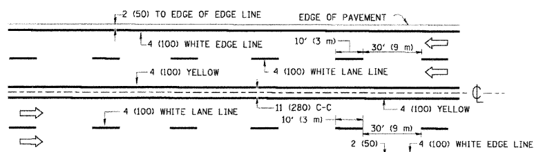
MULTI-LANE UNDIVIDED
