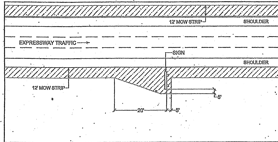
Mowing Detail #4
