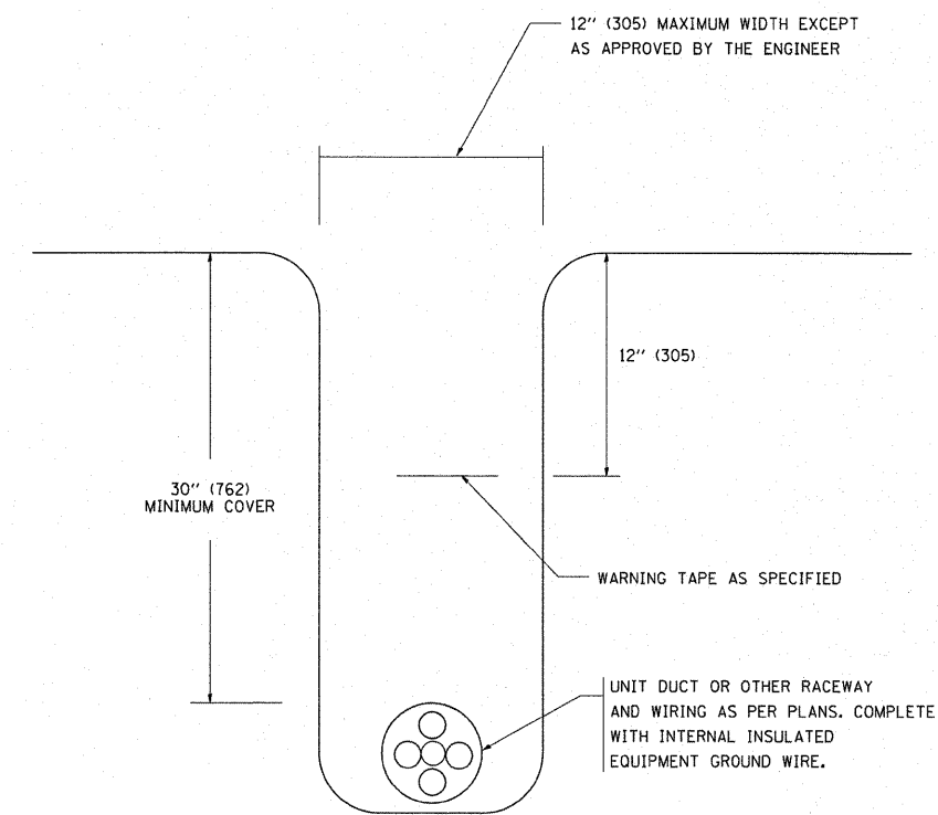
TYPICAL WIRING IN TRENCH DETAIL
