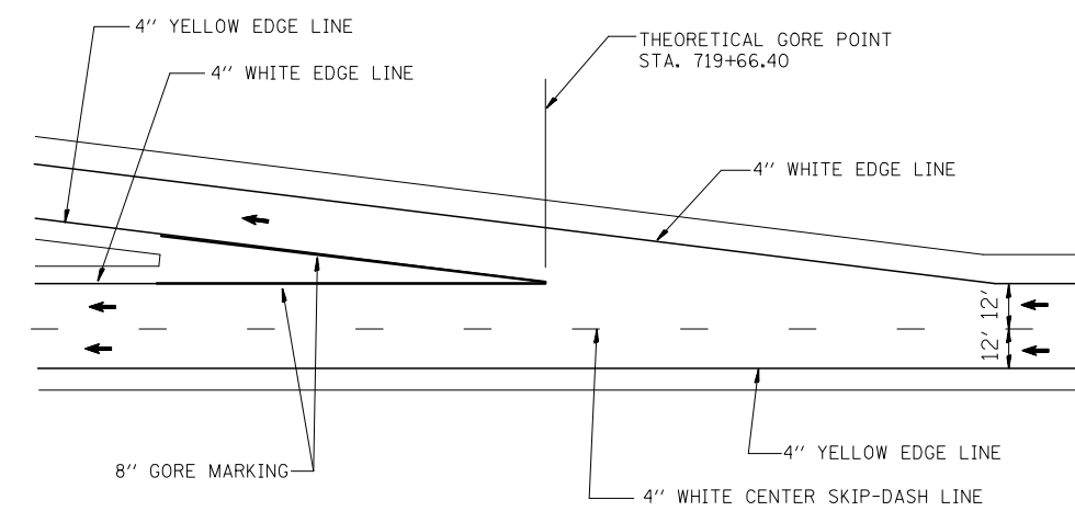
TYPICAL EXIT RAMP MARKINGS
