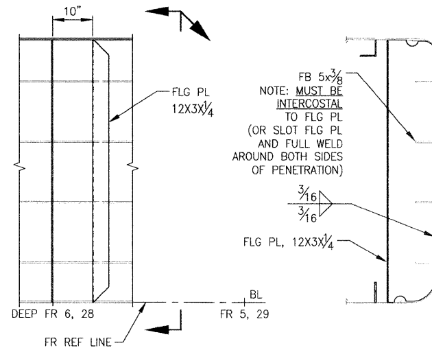
8 FENDER BACKING FRAME DETAIL PORT ONLY SCALE: 3/4" = 1'-0"
