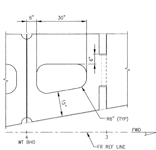
7 DETAIL NT BHD 7-8" OFF CL CUTOUT BETWEEN FR 3 & 4 CUTOUT BETWEEN FR 30 & 31, SIM OPP HAND SCALE: 3/4" = 1'-0"
