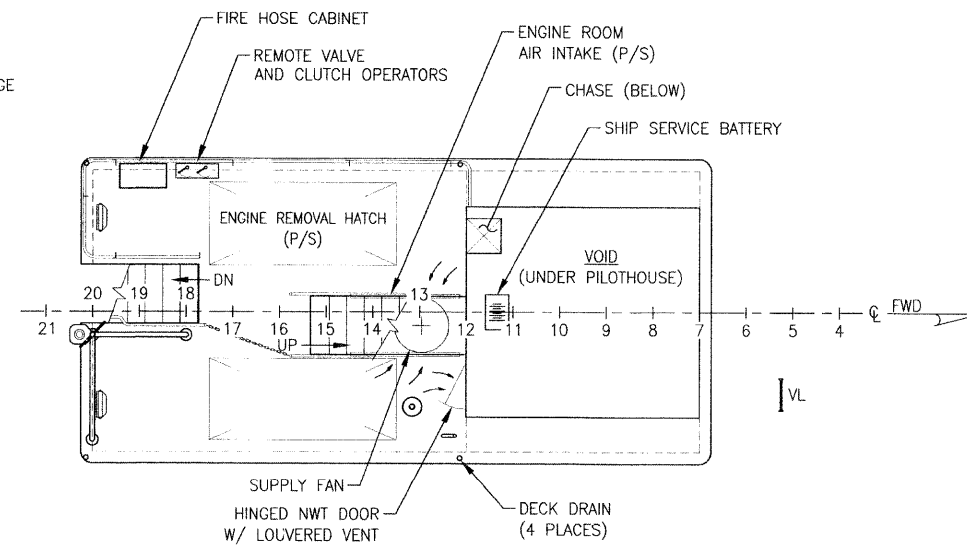
UPPER DECK PLAN SCALE: 1/4" = 1'-0"
