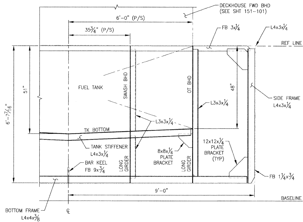
FRAME 7 SECTION
