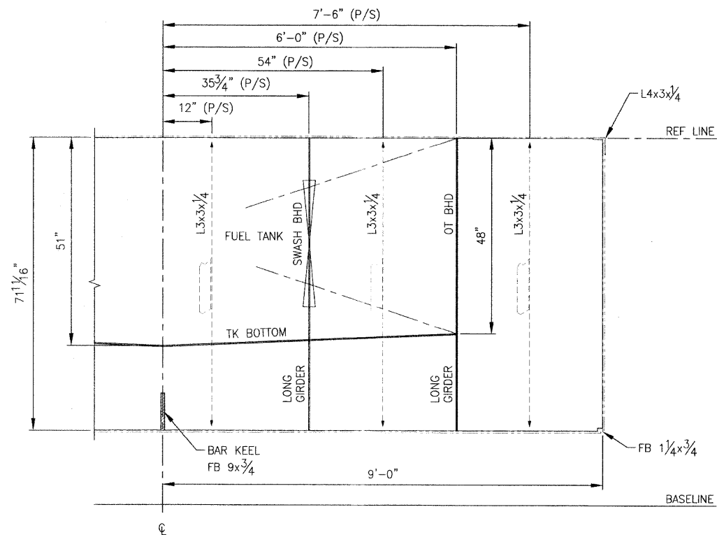
FRAME 6 SECTION
