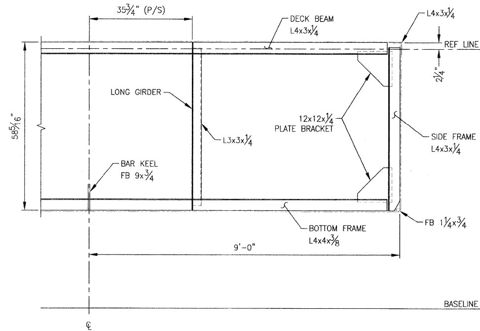
FRAME 4 SECTION
