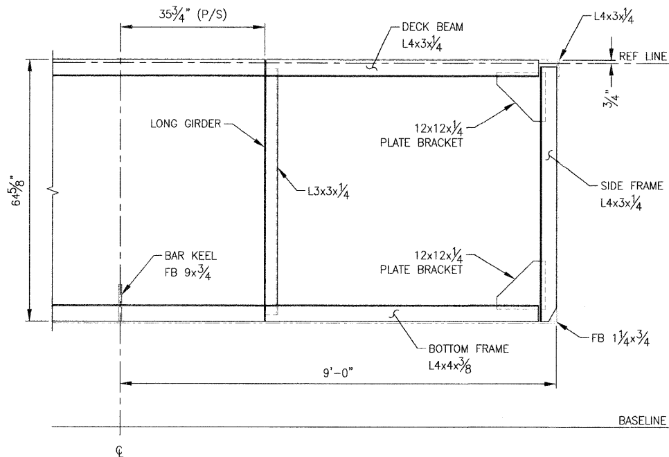
FRAME 5 SECTION
