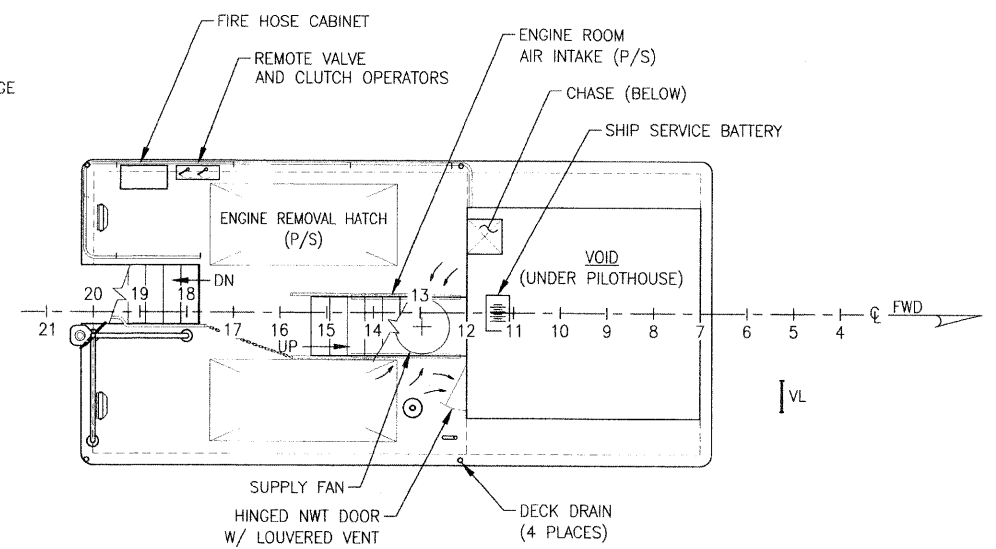
UPPER DECK PLAN SCALE: 1/4" = 1'-0"
