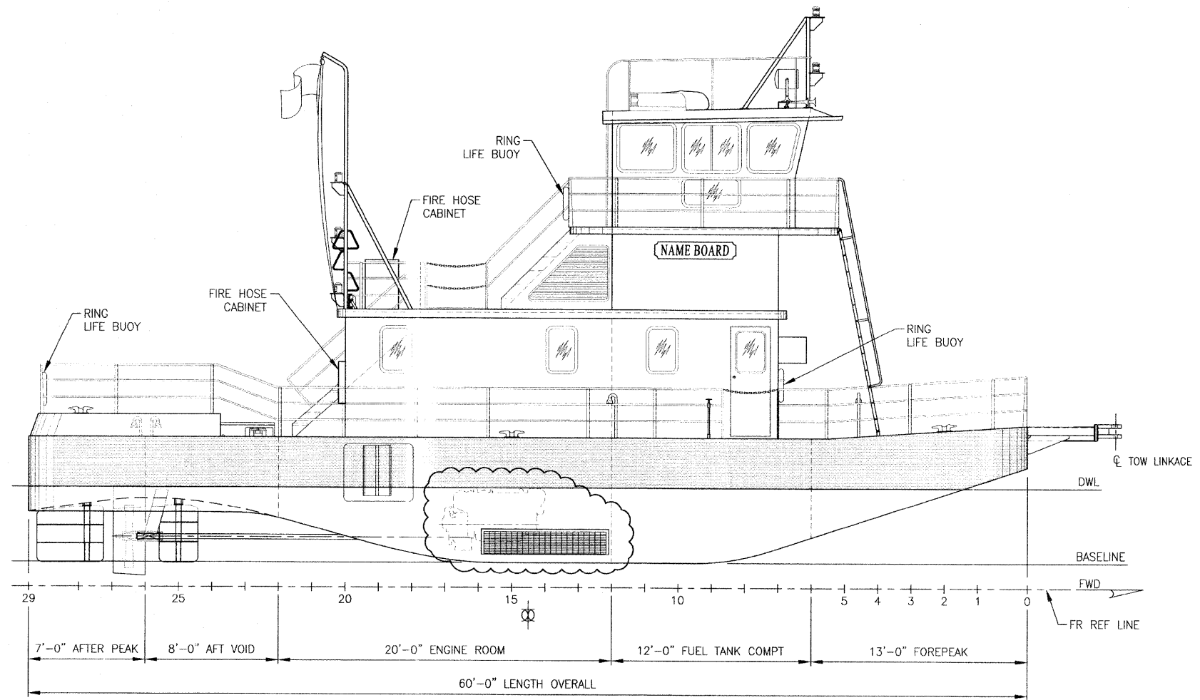
STARBOARD PROFILE SCALE: 1/4" = 1'-0"
