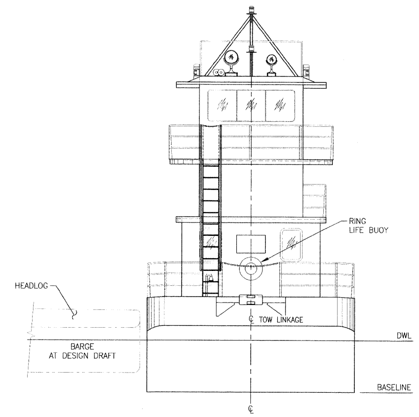
BOW ELEVATION SCALE: 1/4" = 1'-0"
