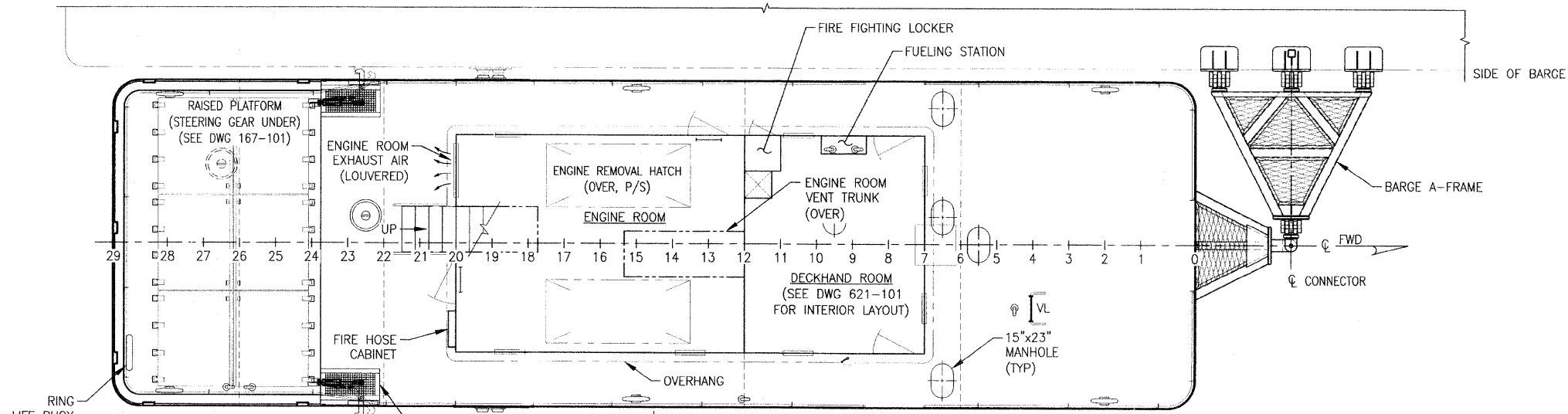
MAIN DECK PLAN SCALE: 1/4" = 1'-0"
