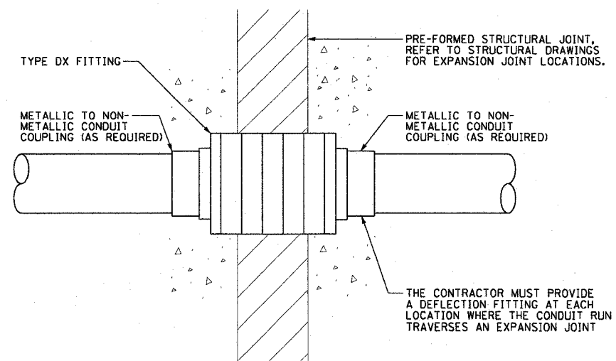
ME-08B CONDUIT DEFLECTION FITTING DETAIL DEFLECTION FITTING, O-Z/GEDNEY DX OR APPROVED EQUAL NOT TO SCALE
