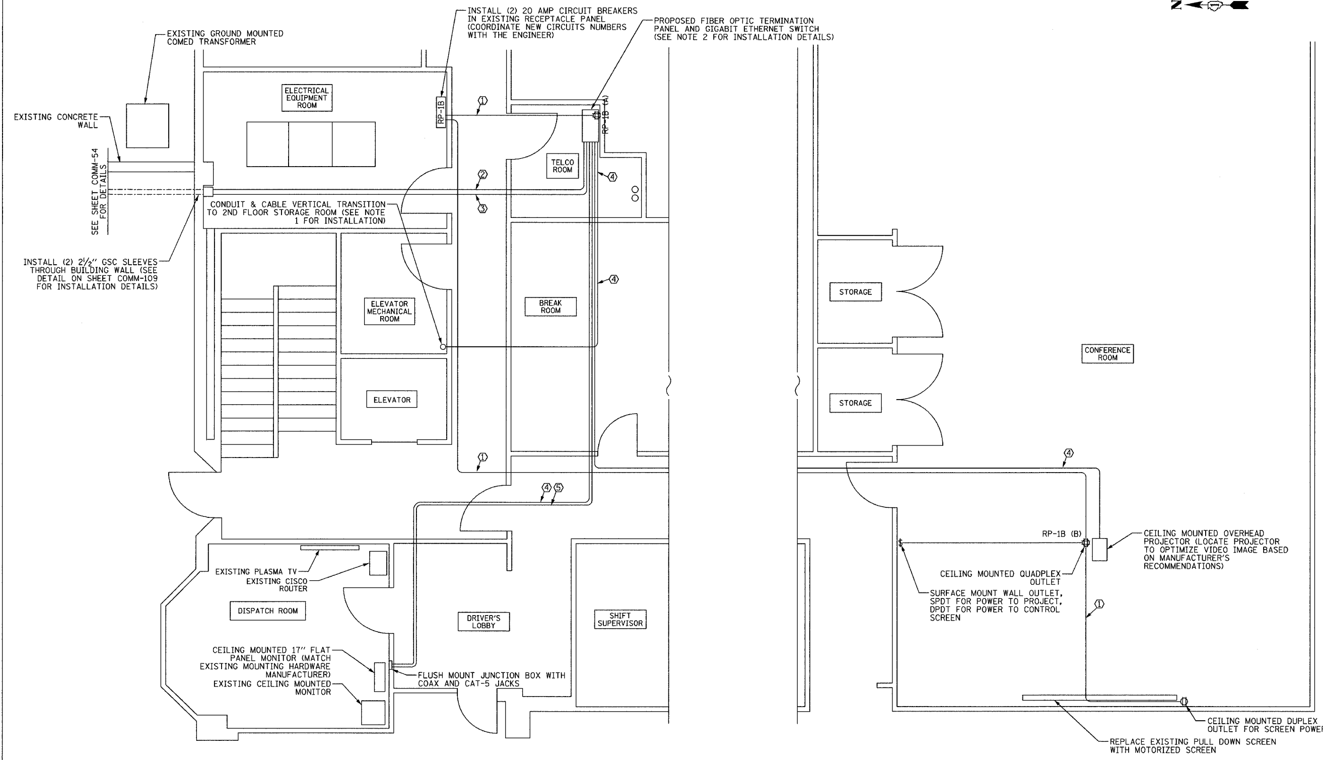
PARTIAL FIRST FLOOR PLAN NOT TO SCALE
